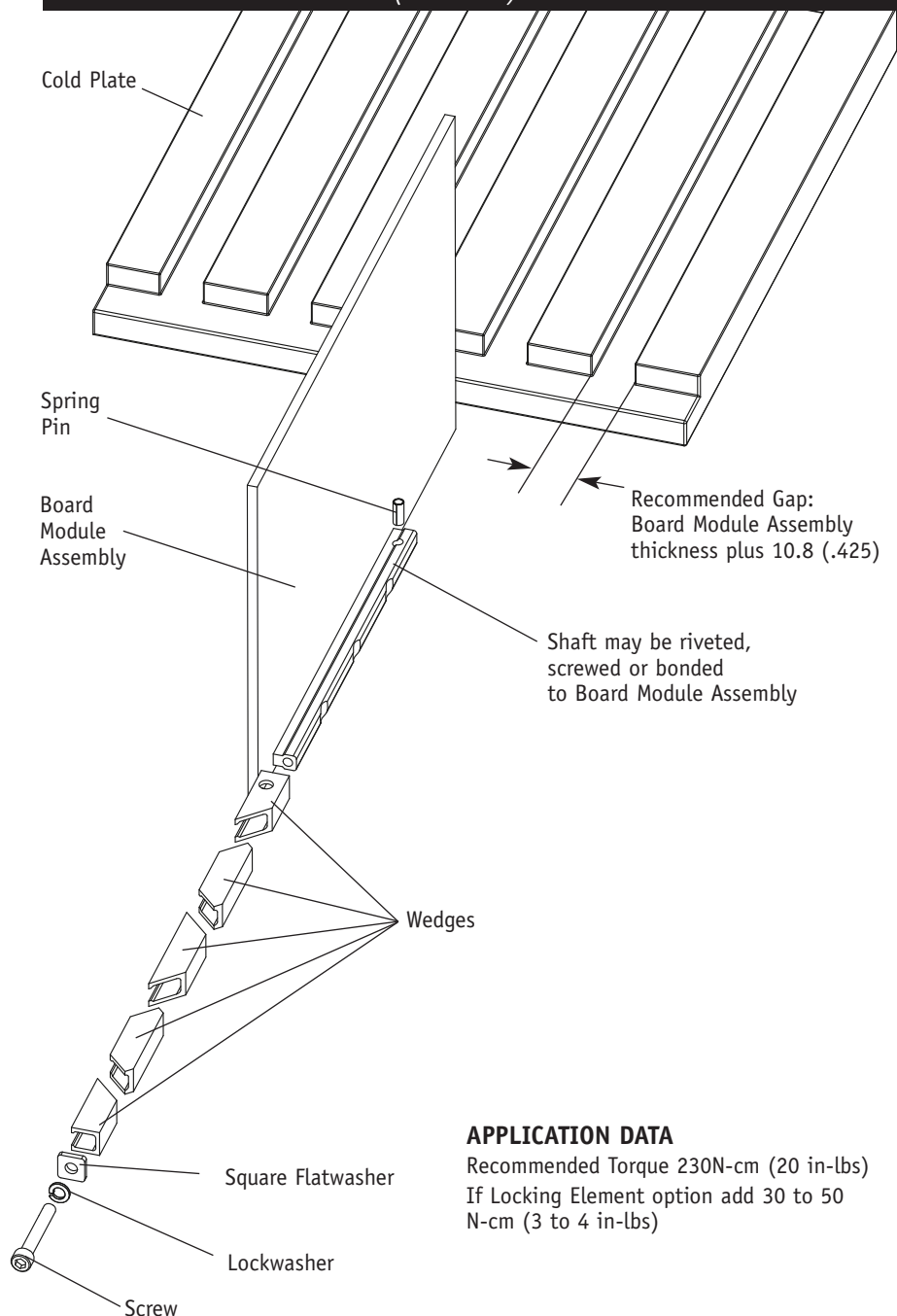
Series 280 - "Card-Lok" Retainer (Cold Plate)
