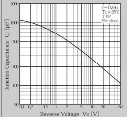
Junction Capacitance
