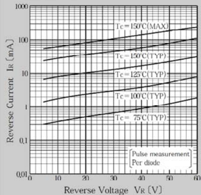
Reverse Current
