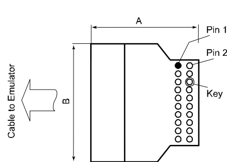
FIGURE 31 Dimensions of the 20-pin CTI20 probe. Top view. A = 27.0 mm (1.06 in.) B = 17.8 mm (0.70 in.).
