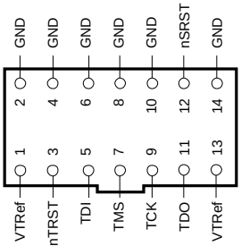
FIGURE 4 The pinout of the 14-pin JTAG probe for ARM. Top view.
