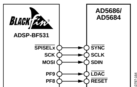
Figure 43. ADSP-BF531 Interface
