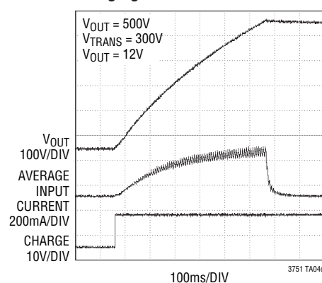
Charging Waveform
