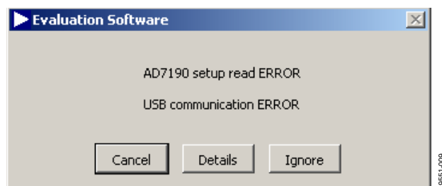
Figure 9. Configuration Tool
