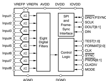
ADS1178
