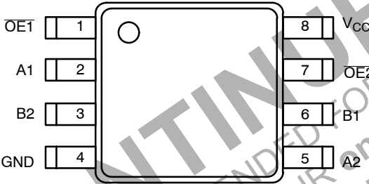
Figure 3. US8/Micro8 (Top View)
