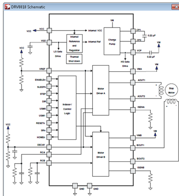
Figure 21. Schematic
