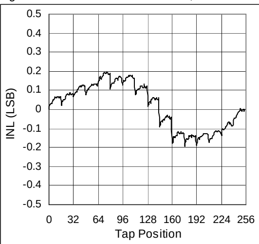
Figure 8. INL vs. TAP Position 100k \Omega , Divider Mode
