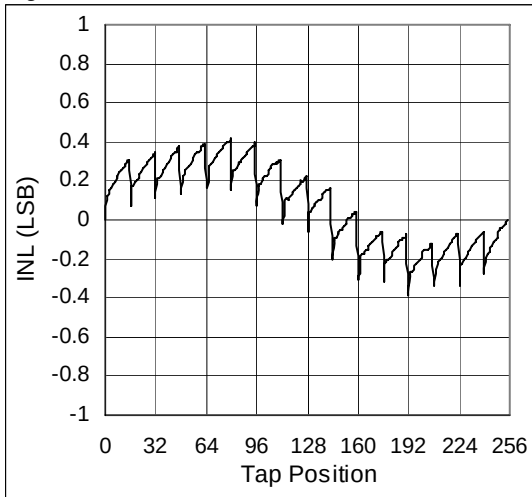
Figure 6. INL vs. TAP Position 50k \Omega , Divider Mode
