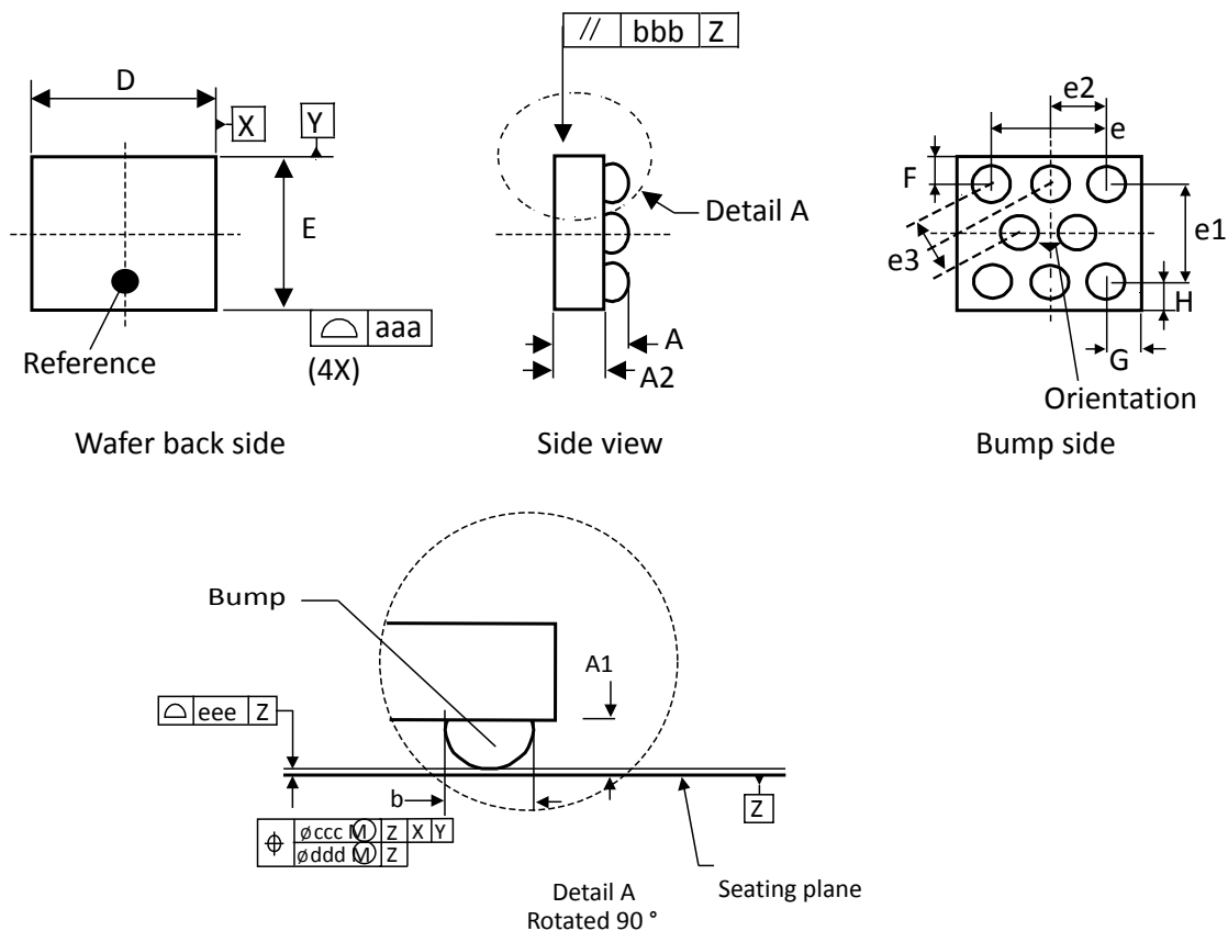
Figure 29. WLCSP8 - Outline
