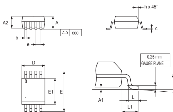
Figure 23. SO8N – Outline
