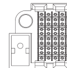
Part Number 120666 50 Position Left Feed-Through ESD/HDI Guide Pin
