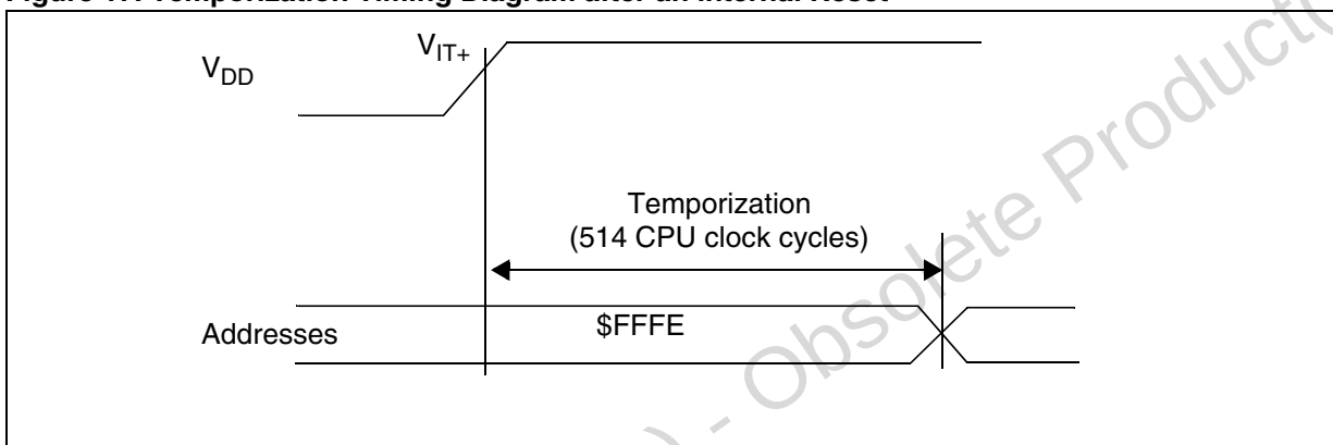
Figure 18. Reset Timing Diagram
