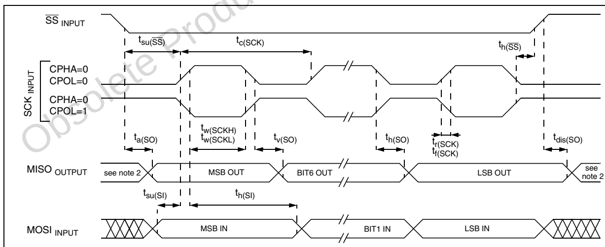
Figure 78. SPI Slave Timing Diagram with CPHA=0 3)
