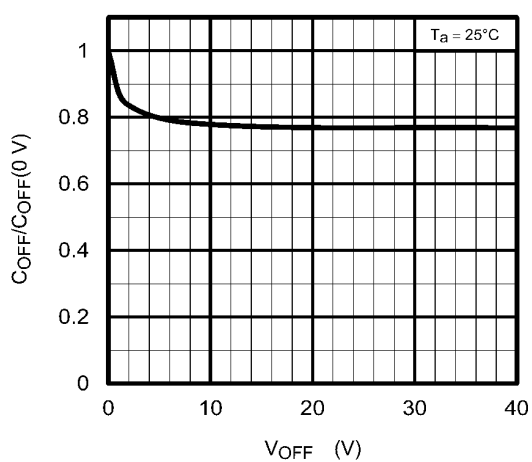
図 12.1.11 C_{OFF}/C_{OFF(0V)} - V_{OFF}
