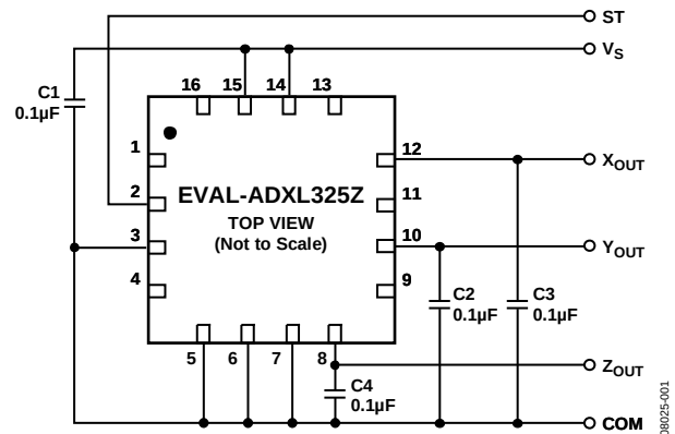
Figure 1. Schematic
