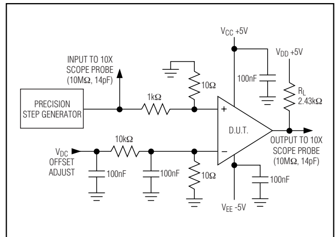
Figure 5. Response-Time Setup
