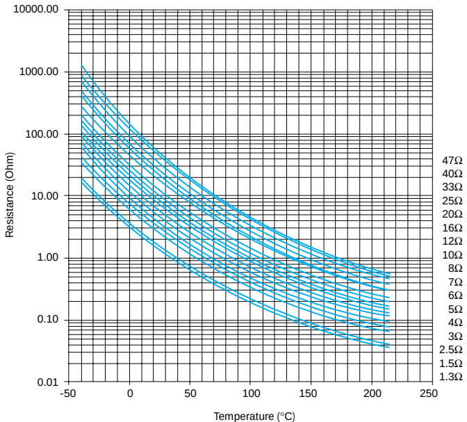
TYPICAL RESISTANCE/TEMPERATURE CHARACTERISTICS FOR TYPE NF15
