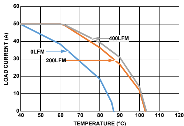
FIGURE 25. 12V_{IN} TO 5V_{OUT} , f_{SW} = 533\text{kHz}
