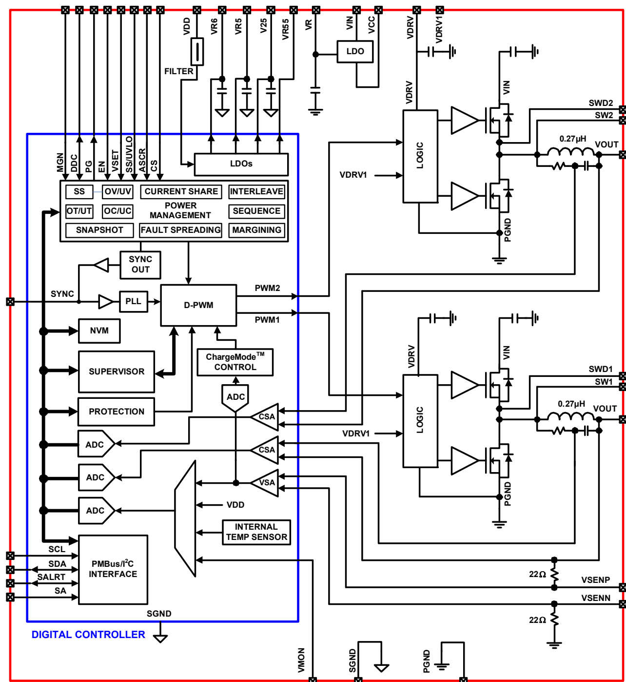
FIGURE 3. INTERNAL BLOCK DIAGRAM
