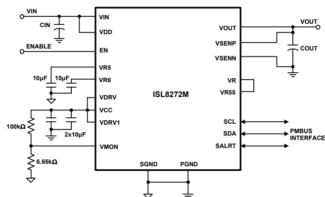
FIGURE 1. 50A APPLICATION CIRCUIT
