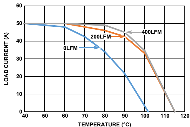
FIGURE 23. 5V_{IN} TO 3.3V_{OUT} , f_{SW} = 300\text{kHz}
