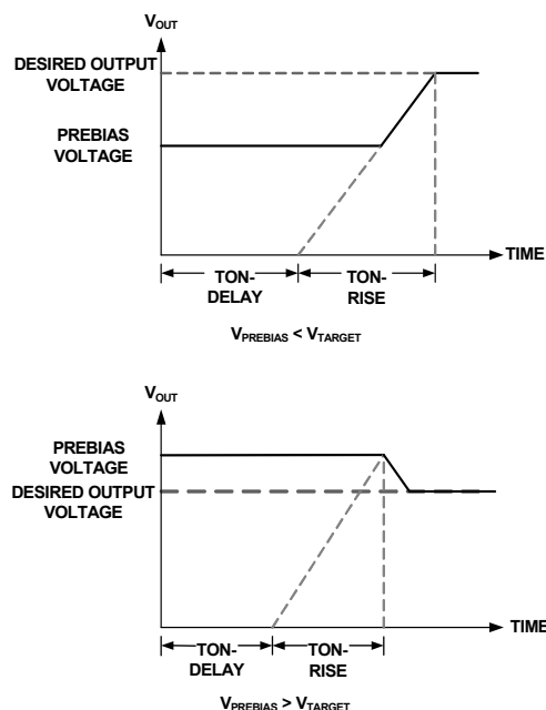
FIGURE 26. OUTPUT RESPONSES TO PREBIAS VOLTAGES
