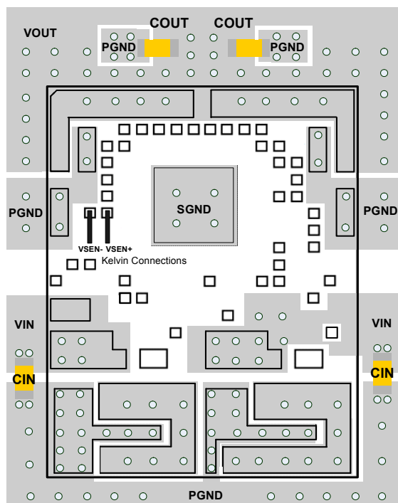
FIGURE 29. RECOMMENDED LAYOUT
