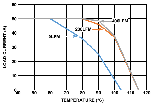
FIGURE 19. 5V_{IN} TO 1.8V_{OUT} , f_{SW} = 300\text{kHz}
