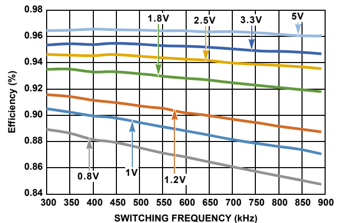
FIGURE 9. EFFICIENCY vs SWITCHING FREQUENCY AT V_{IN} = 9\text{V} , I_{OUT} = 50\text{A} FOR VARIOUS OUTPUT VOLTAGES
