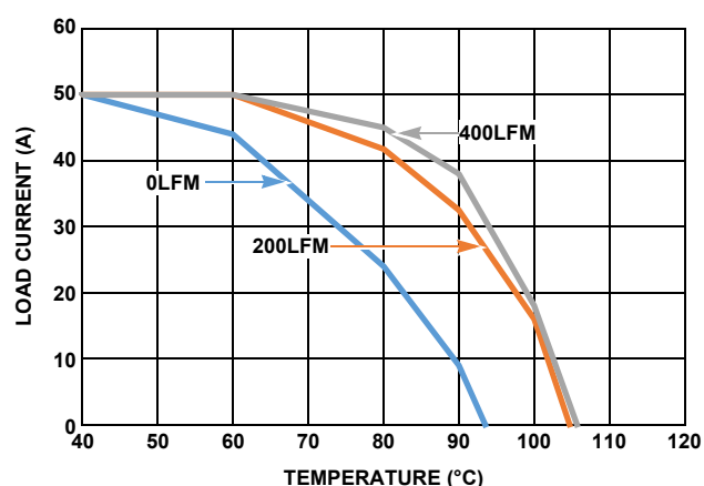
FIGURE 24. 12V_{IN} TO 3.3V_{OUT} , f_{SW} = 533\text{kHz}
