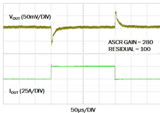
FIGURE 13. 1.8V TRANSIENT RESPONSE. C_{OUT} = 6 \times 100\mu F CERAMIC + 2 \times 470\mu F POSCAP
