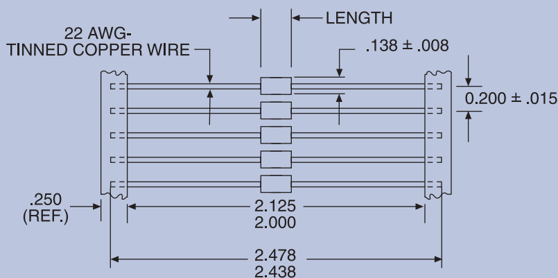
OUTLINE DRAWING
