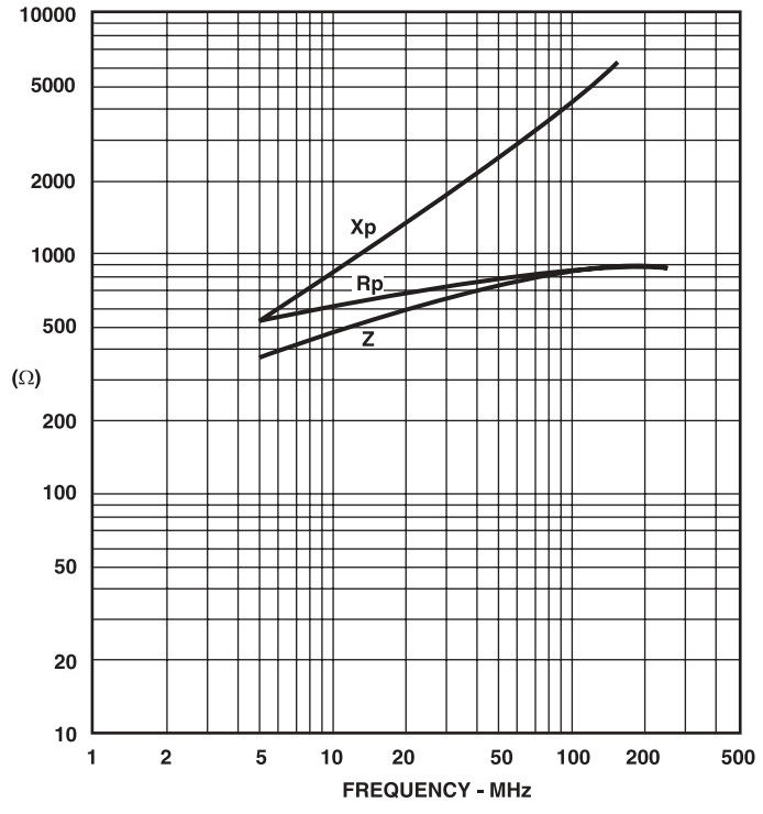
11-081-J 6 TURNS
