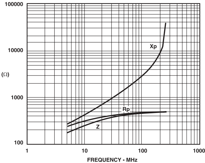
12-340-G 3 TURNS
