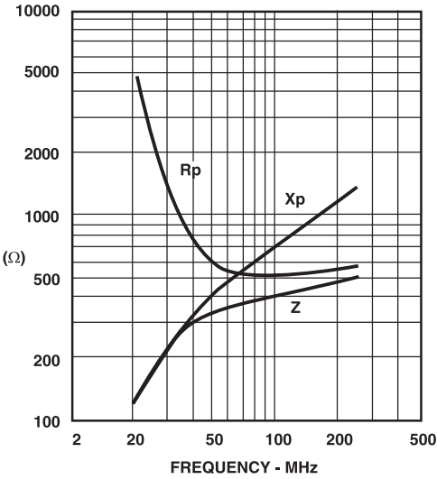
12-345-K 2 TURNS
