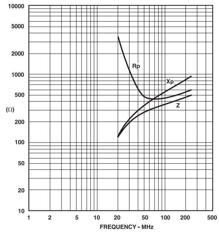
11-120-K 4 TURNS
