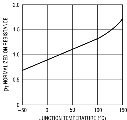
Figure 12. Normalized R_{DS(ON)} vs Temperature
