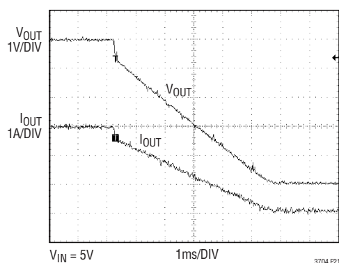
Figure 21. Soft-Start for the Circuit in Figure 15
