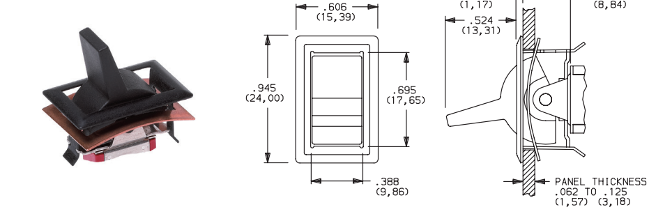
J21 LEVER WITH FRAME
