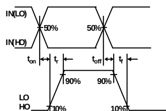
Figure 3. Switching Time Waveform Definitions
