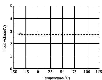
Figure 15b. Logic 1 Input Voltage vs Temperature
