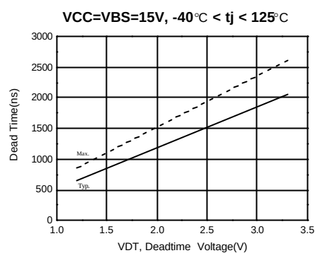
Figure 2. Dead Time VS V_{DT}
