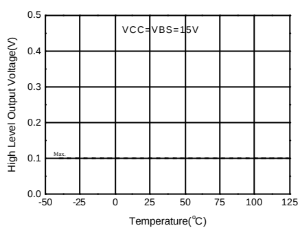
Figure 16a. High Level Output of HO vs Temperature
