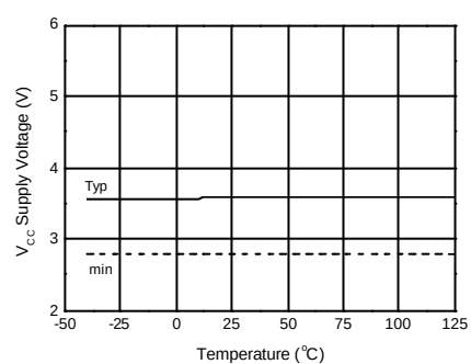
Figure 24b. VCC UnderVoltage Threshold(-) vs Temperature
