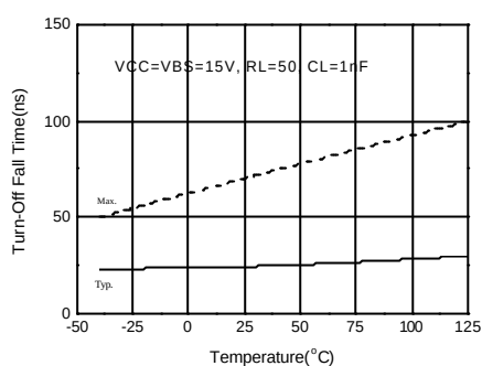
Figure 13a. Turn-Off Fall Time of HO vs Temperature
