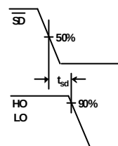
Figure 4. Shutdown Waveform Definitions
