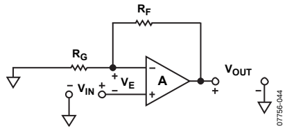
Figure 41. Noninverting Configuration
