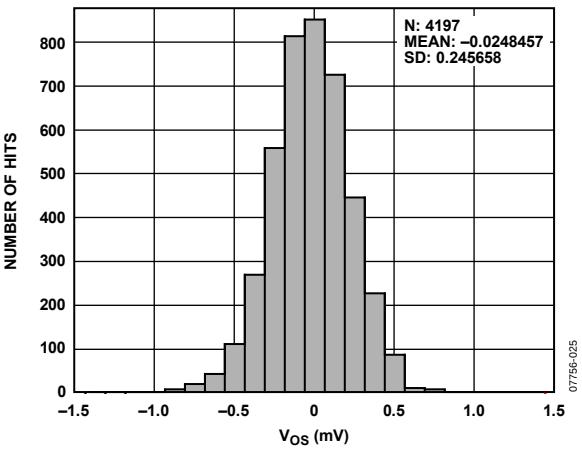
Figure 34. Input Offset Voltage Histogram
