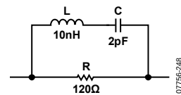
Figure 48. RLC Circuit
