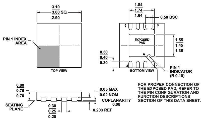
Figure 58. 8-Lead Lead Frame Chip Scale Package [LFCSF]
