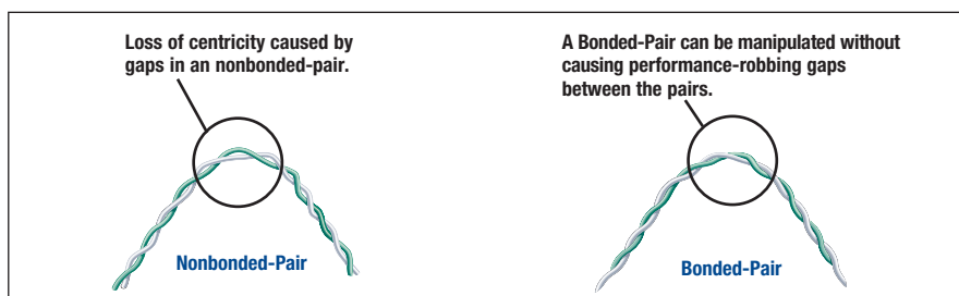
Figure 2: The slightest manipulation of a nonbonded-pair (left) can cause gaps between the conductors of the pair and impair electrical performance. Gaps cannot form between the conductors in a Bonded-Pair (right), resulting in consistent electrical performance.
