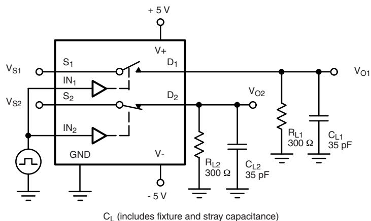
Figure 2. Break-Before-Make (DG613A)
