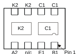
Bottom View Pin-Out
