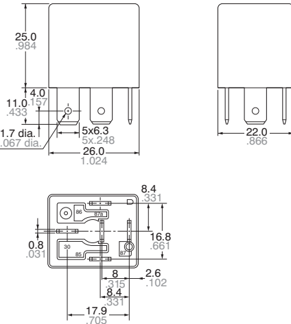
External dimensions
