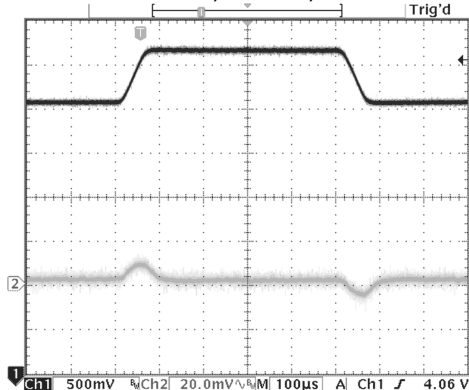
Line Transient (LDO1) 3.6 - 4.5 Vin, 3.3 Vout, 150 mA load
