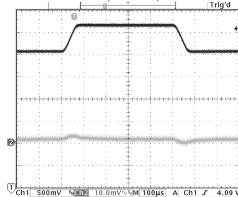
Line Transient (LDO2) 3 - 4.2 Vin, 1.8 Vout, 150 mA load
