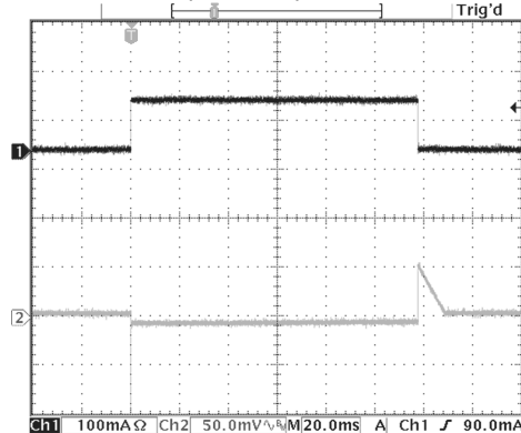
Load Transient (LDO1) 3.6 Vin, 3.3 Vout, 0 – 100 mA load
