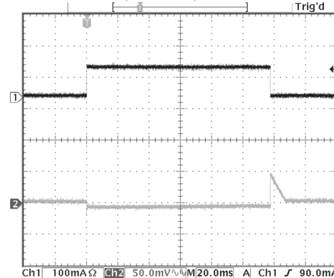
Load Transient (LDO2) 3.6 Vin, 1.8 Vout, 0 – 100 mA load
