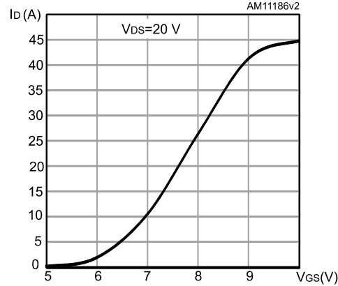
Figure 9: Transfer characteristics
