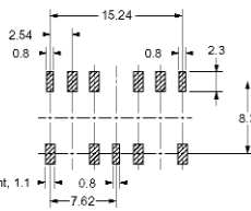
Mounting Dimensions (Top View) Tolerance: \pm 0.1 mm
