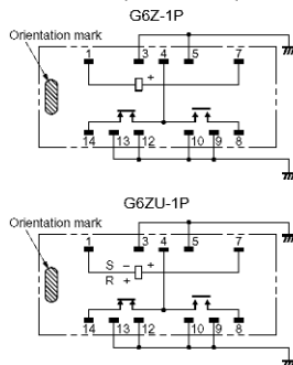
Terminal Arrangement/Internal Connections (Bottom View)
