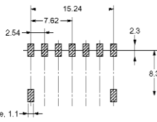
Mounting Dimensions (Top View) Tolerance: \pm 0.1 mm
