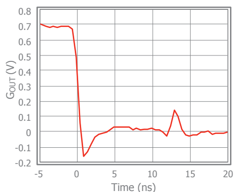
Figure 8. Matched t_F
