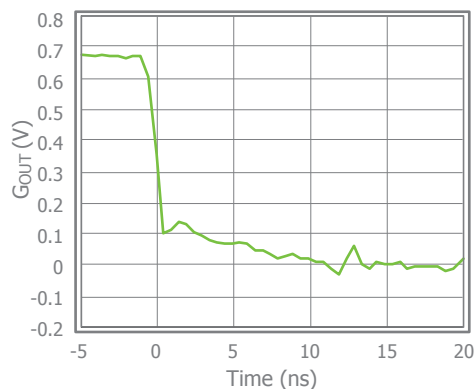
Figure 7. Unmatched t_F
