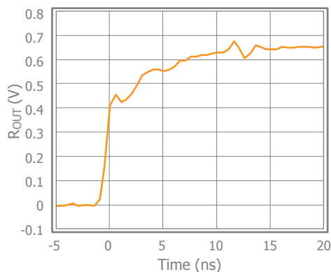
Figure 5. Unmatched t_R
