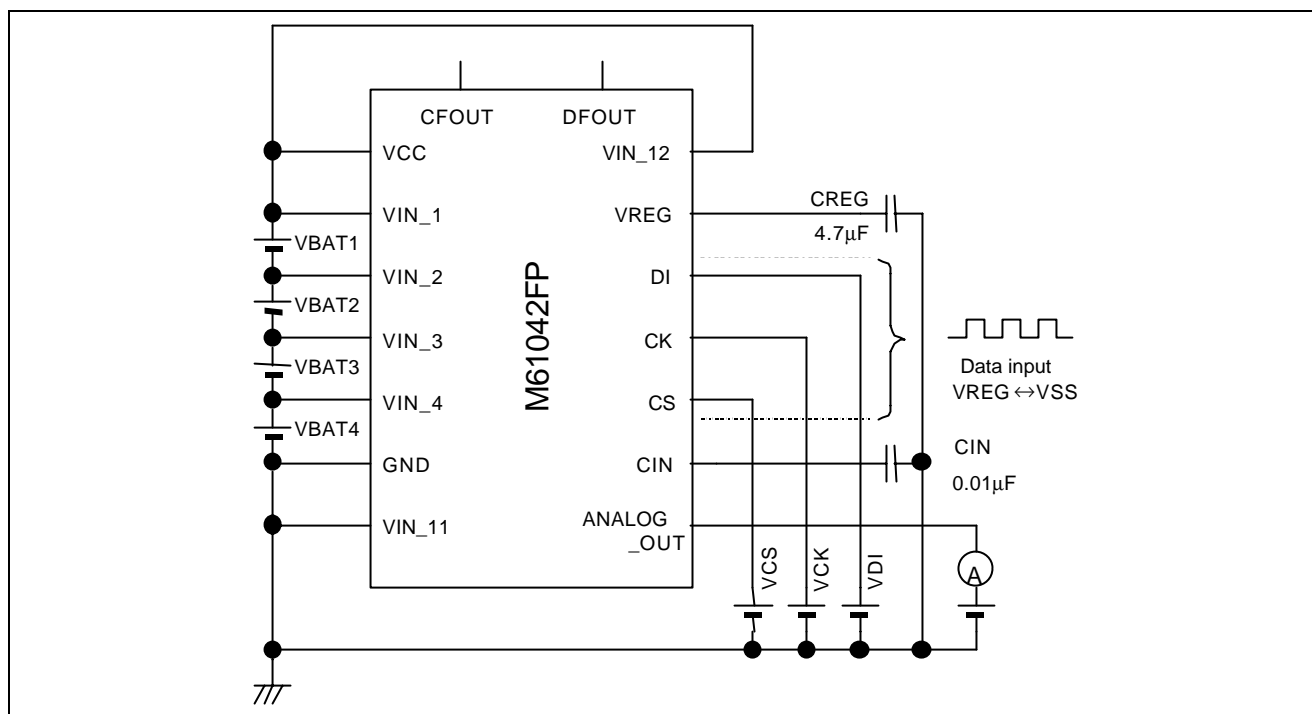
Circuit 6
