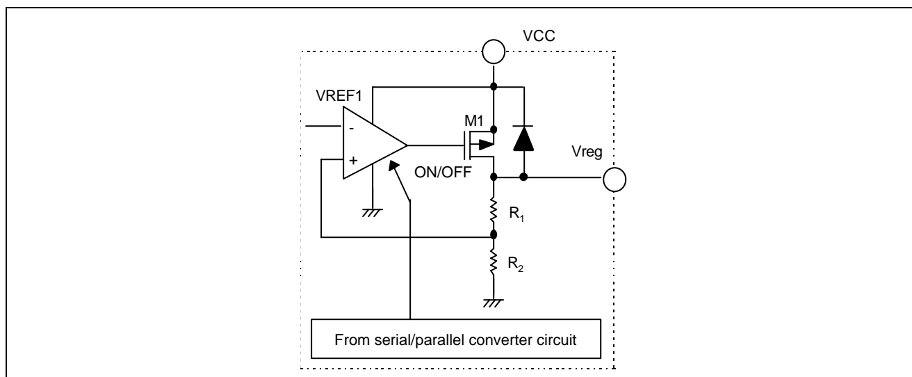
Figure 10 Series Regulator
