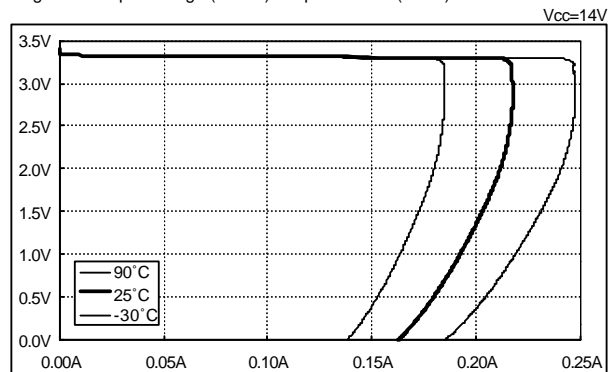
Regulator Output Voltage (VREG)-Output Current (IREG) Characteristics
