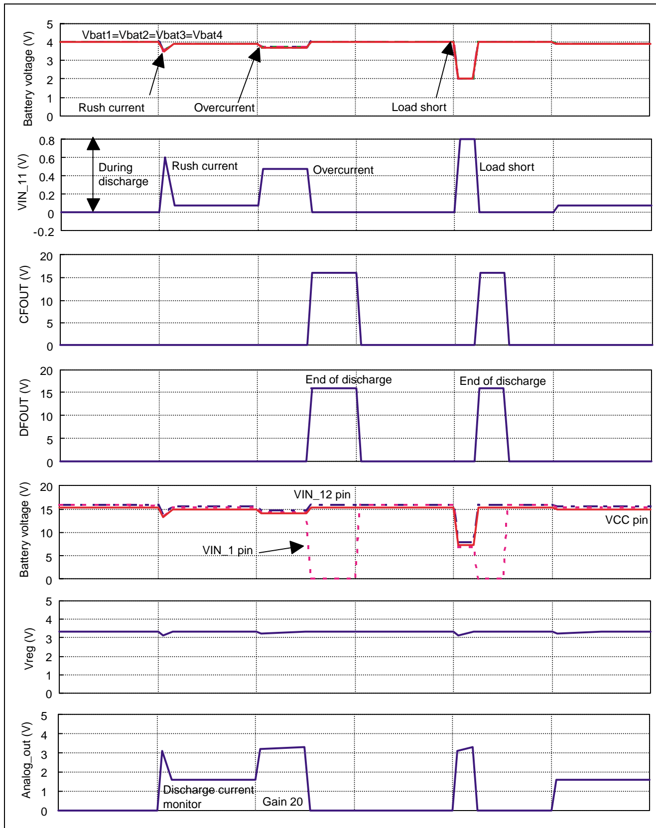
Figure 16 Overcurrent Sequence
