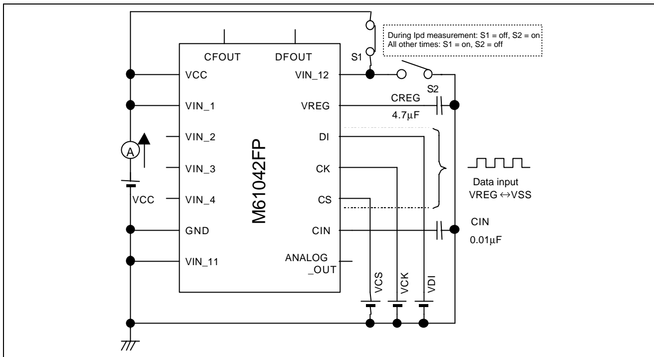
Circuit 1
