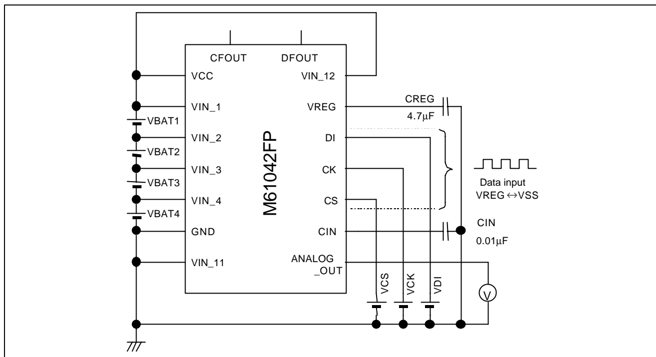
Circuit 5
