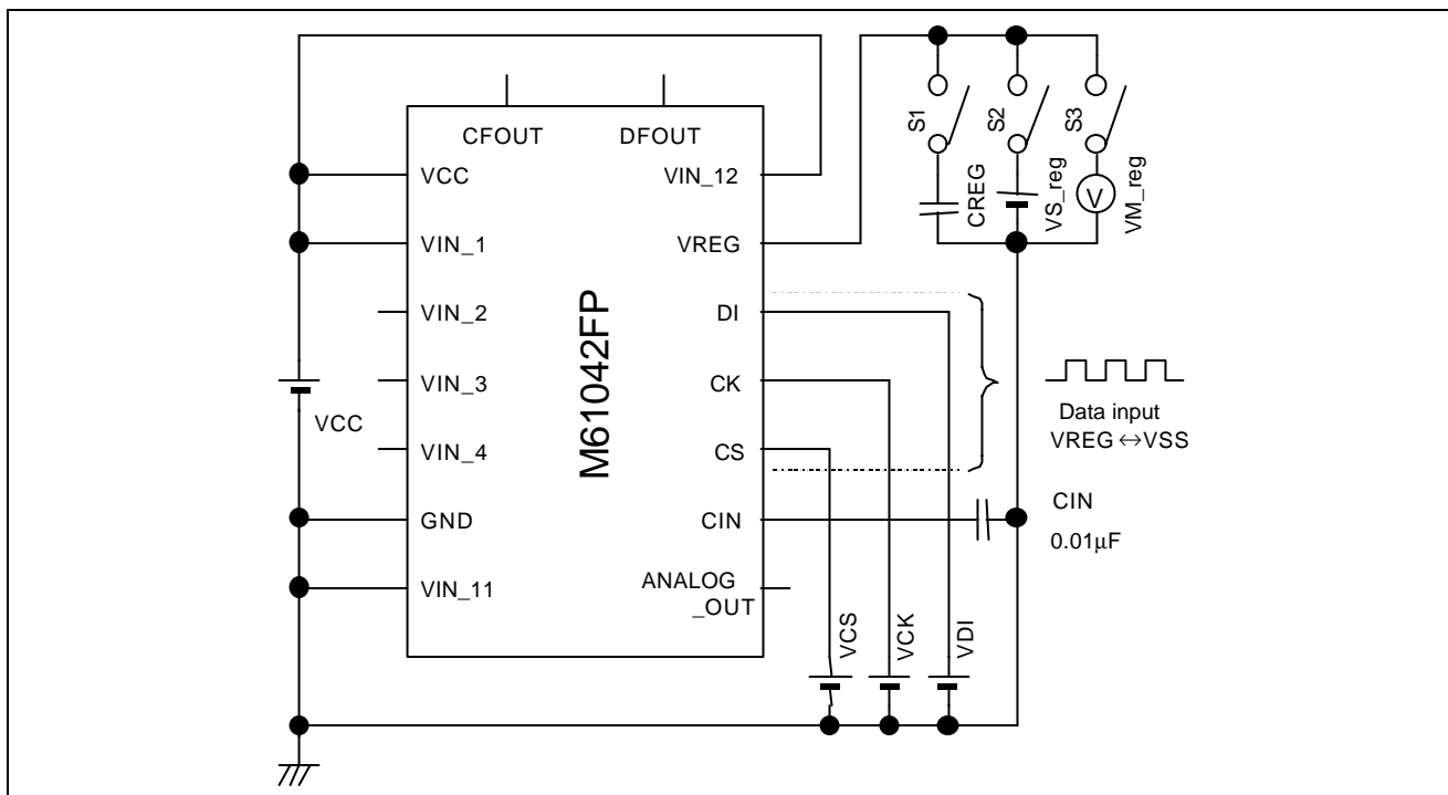
Circuit 2
