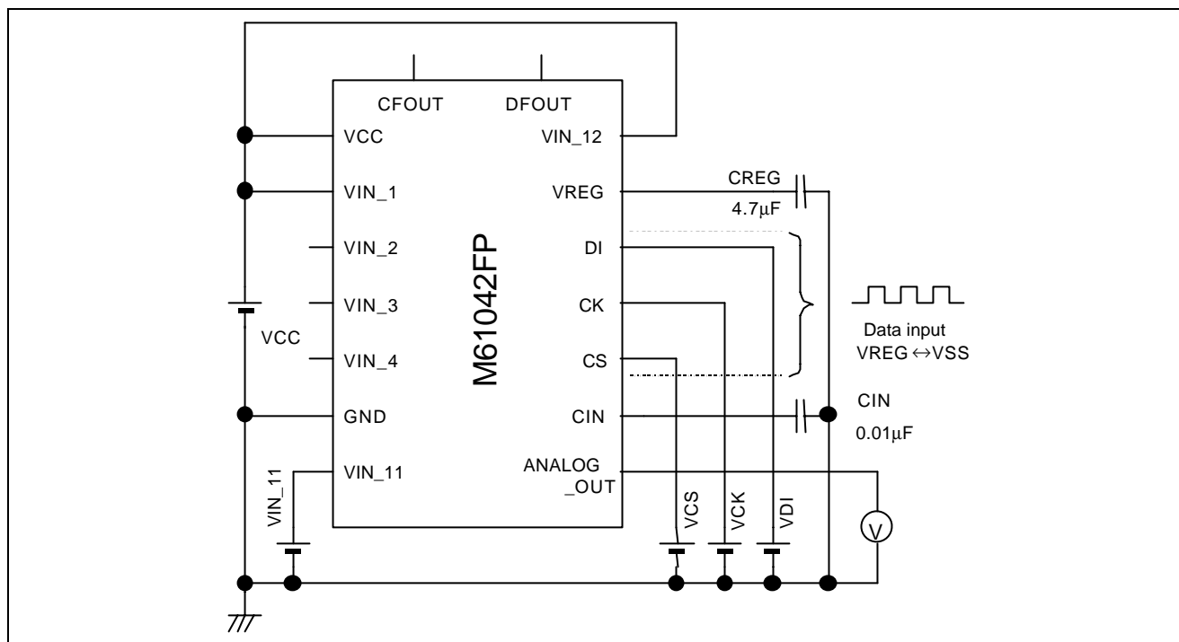
Circuit 7
