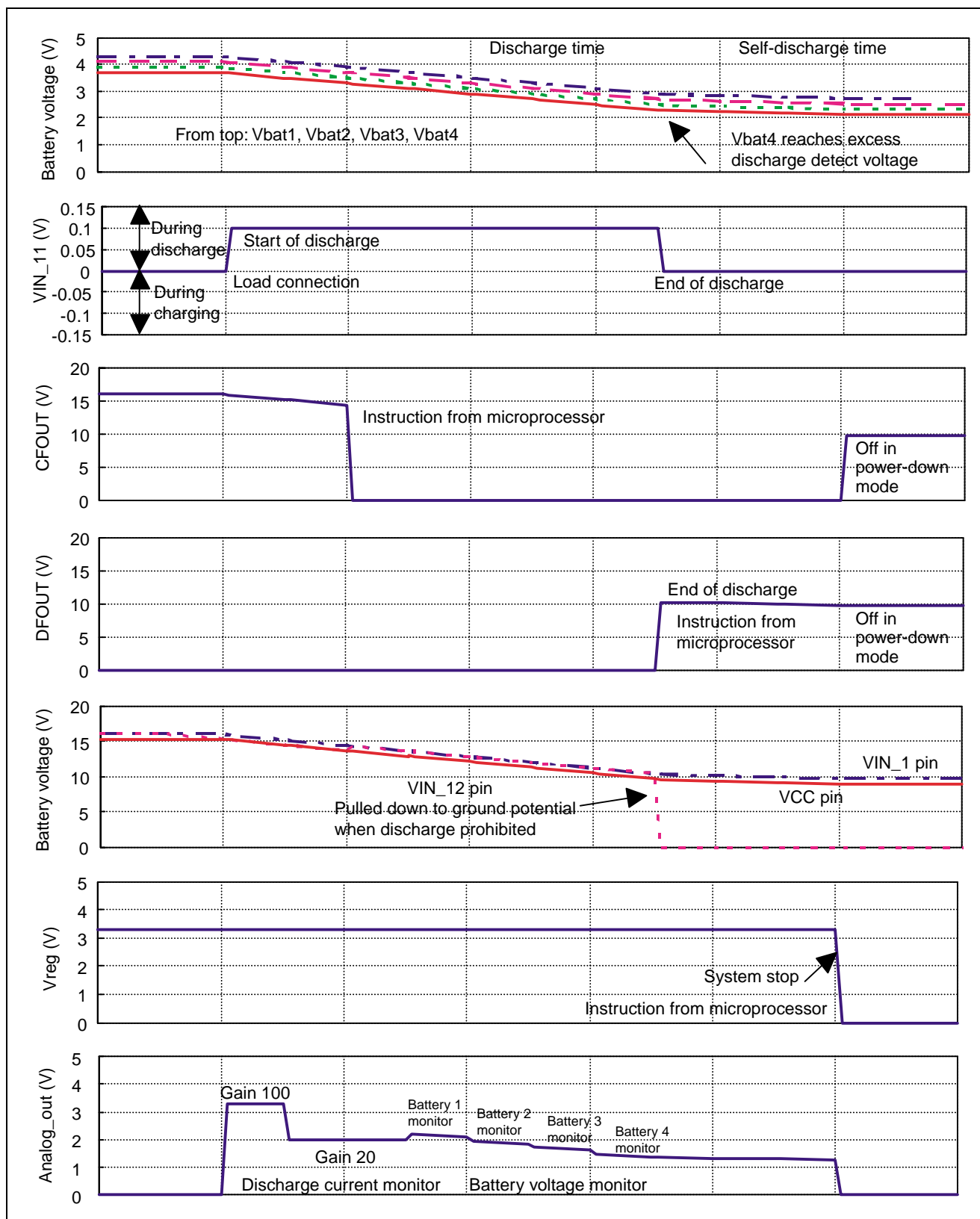
Figure 15 Discharge Sequence
