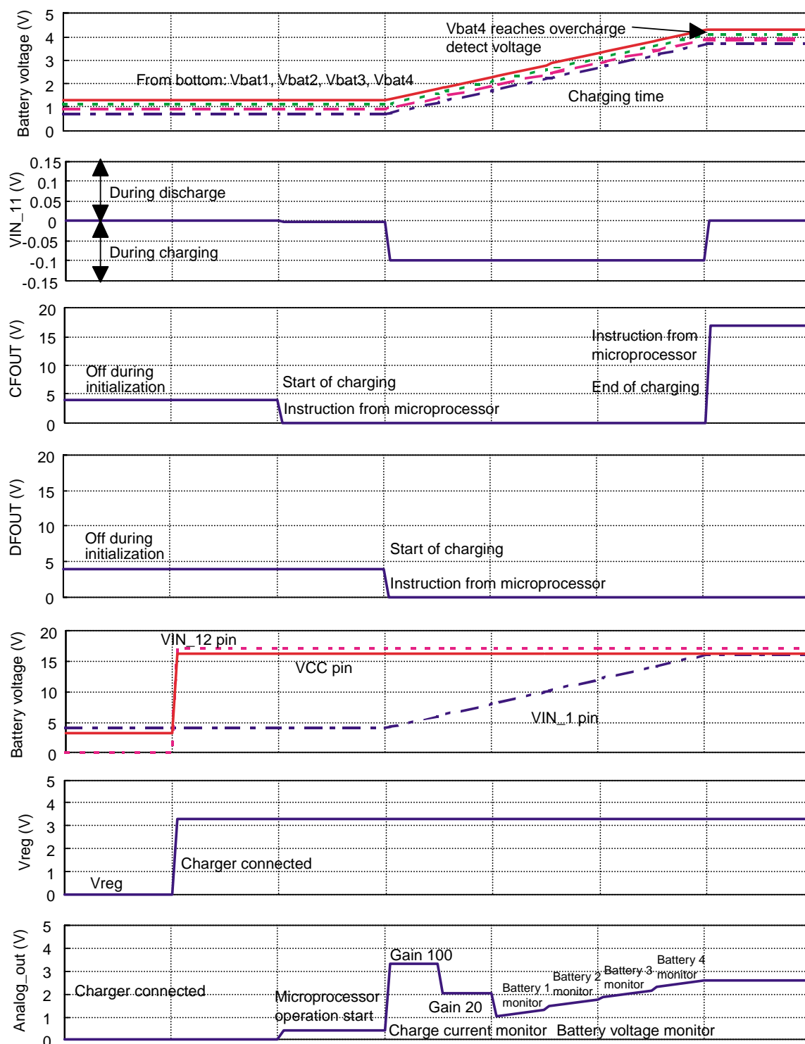
Figure 14 Charging Sequence
