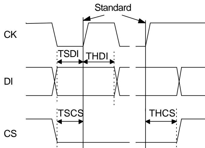
Figure 5 Interface Block Timing Definitions
