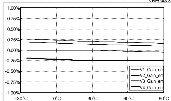
Battery Voltage Amplification Ratio 1 (Gamp1)-Temperature (Ta) Characteristics VREG=3.3V
