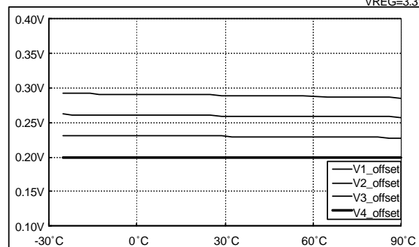
Battery Voltage Input Offset Voltage (VOFF1)-Temperature (Ta) Characteristics VREG=3.3V
