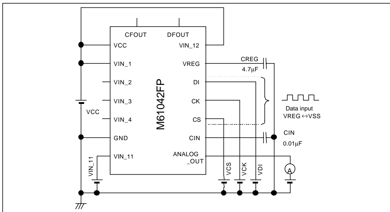
Circuit 8
