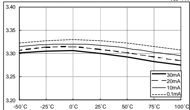
Regulator Output Voltage (VREG)-Temperature (Ta) Characteristics
