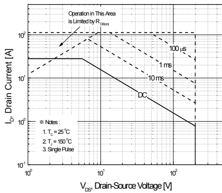
Figure 9-1. Maximum Safe Operating Area for FQP32N20C
