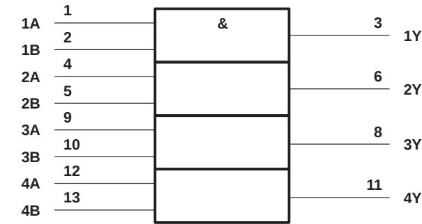
logic symbol†
