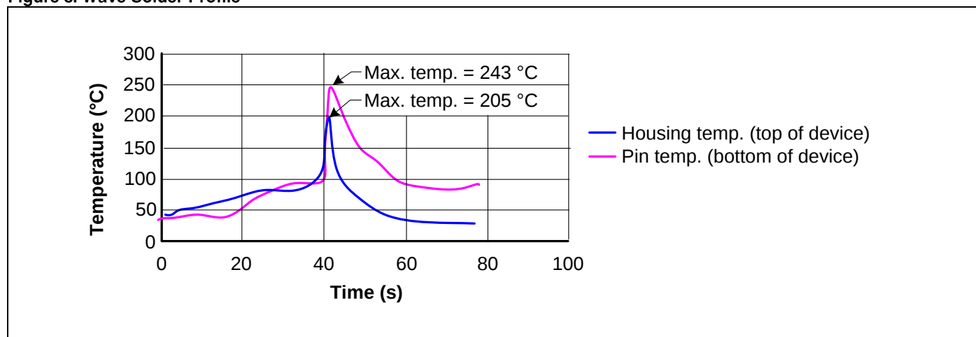
Figure 8. Wave Solder Profile
