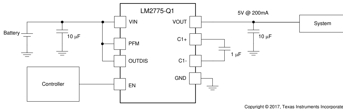
Figure 8-1. Typical LM2775-Q1 Configuration
