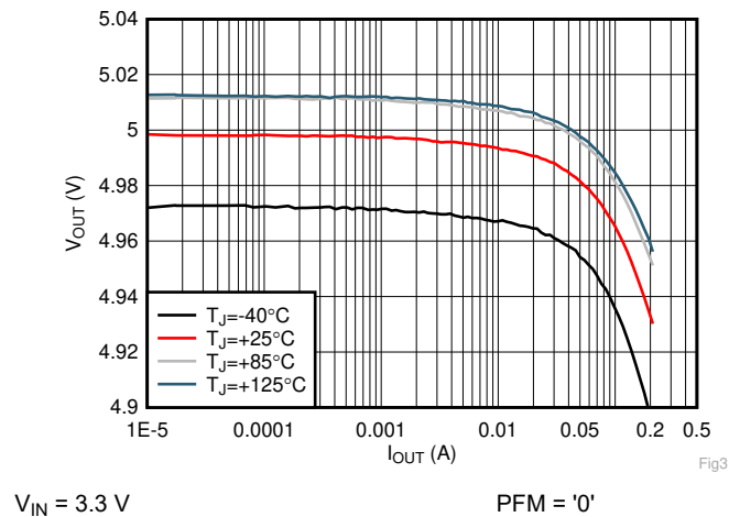
Figure 8-4. Load Regulation
