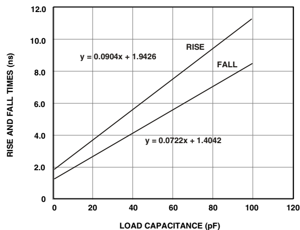
Figure 31. Typical Output Rise/Fall Time (20%-80%, V DDEX = Max)
