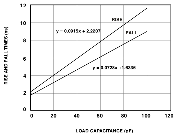
Figure 32. Typical Output Rise/Fall Time (20%-80%, V DDEX = Min)
