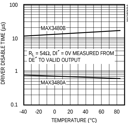
DRIVER DISABLE TIME vs. TEMPERATURE
