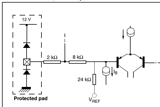
Figure 12. Audio inputs (pins 11, 13, 19, 20, 22, and 23)
