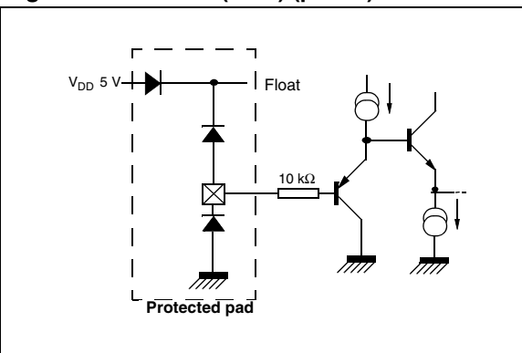
Figure 17. I²C bus (ADD) (pin 54)
