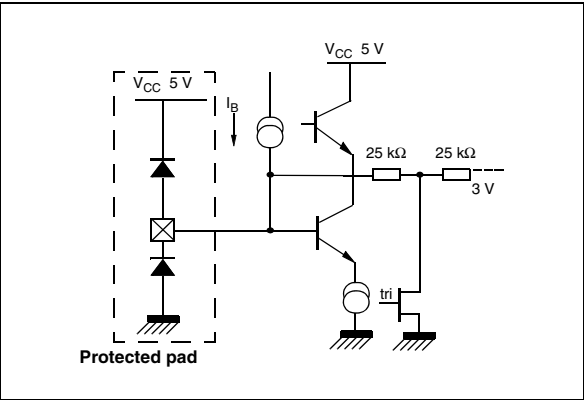
Figure 9. Fast blanking output (pin 49)
