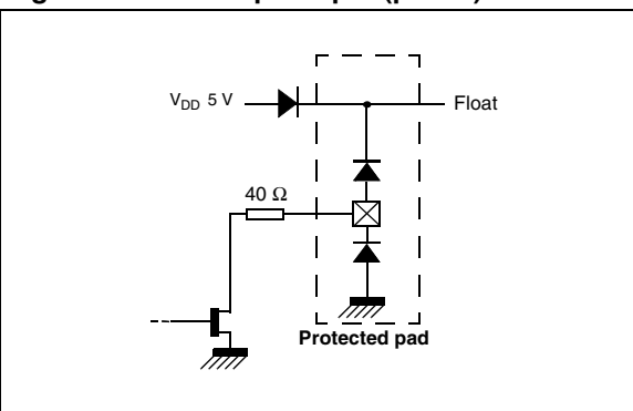
Figure 17. I²C bus (ADD) (pin 54)
