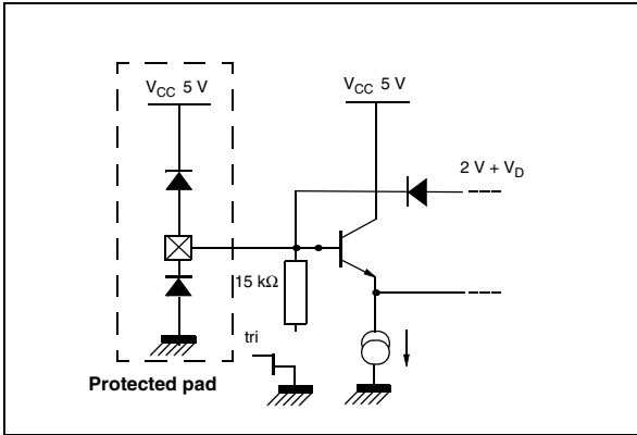
R/C clamped video inputs (pins 10 and 60)
