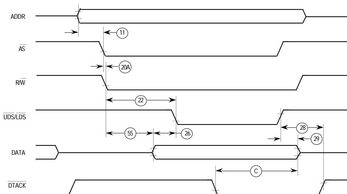
Figure 3-31. Pseudo-Asynchronous Write Cycle
