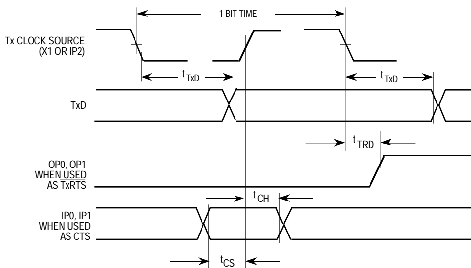
Figure 8-15. Transmit Timing
