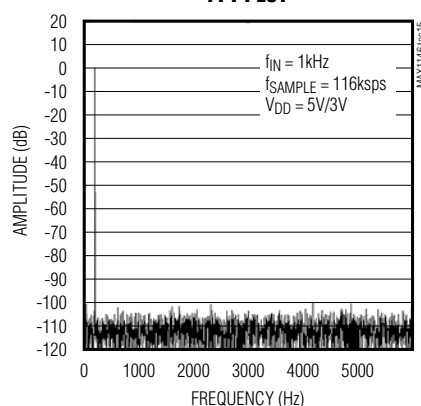
FFT PLOT
