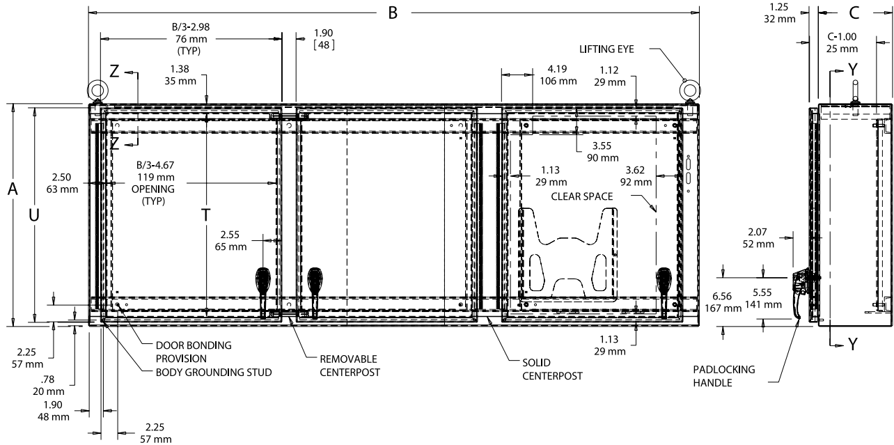
Three-Door Enclosure
