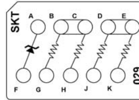
CTJ420E029 Two 10 kOhm Resistors, 1/10 W Two 1.43 kOhm Resistors, 1/10 W One JANTX 1N4954 Zener Diode
