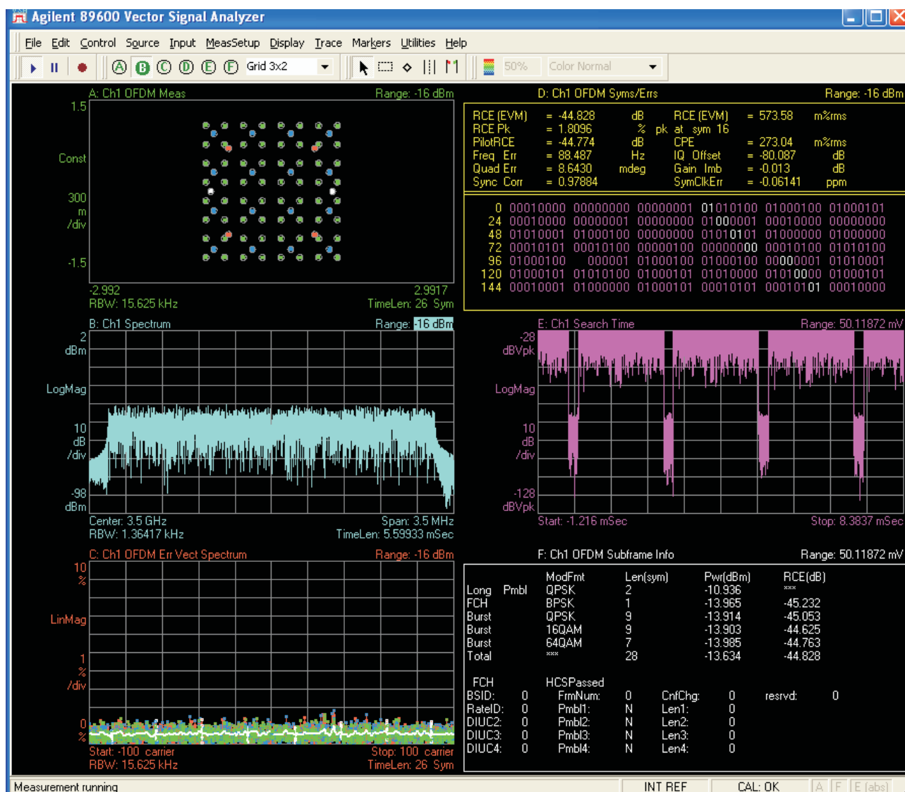
Figure 3. TRF1x22EVM Performance
