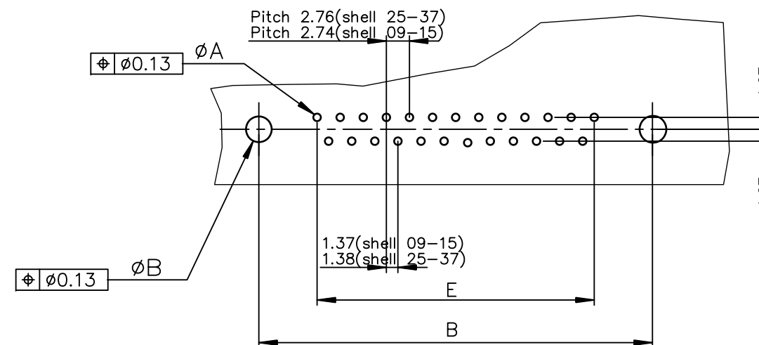
PC card drilling dimensions(after plating) (thickness 1.60 ±0.20 )
