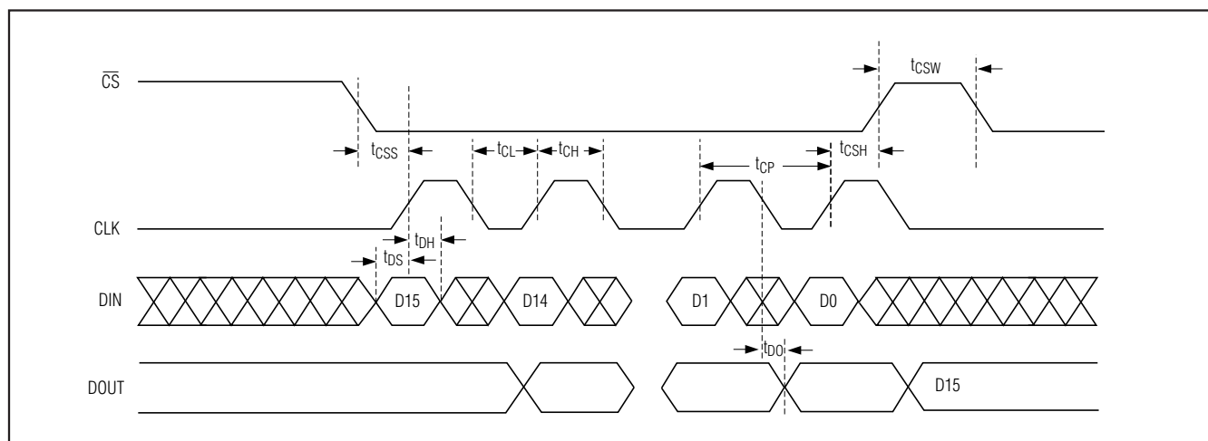
Figure 3. Timing Diagram
