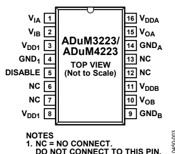
Figure 4. Pin Configuration
