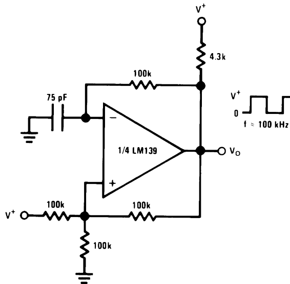
Squarewave Oscillator
