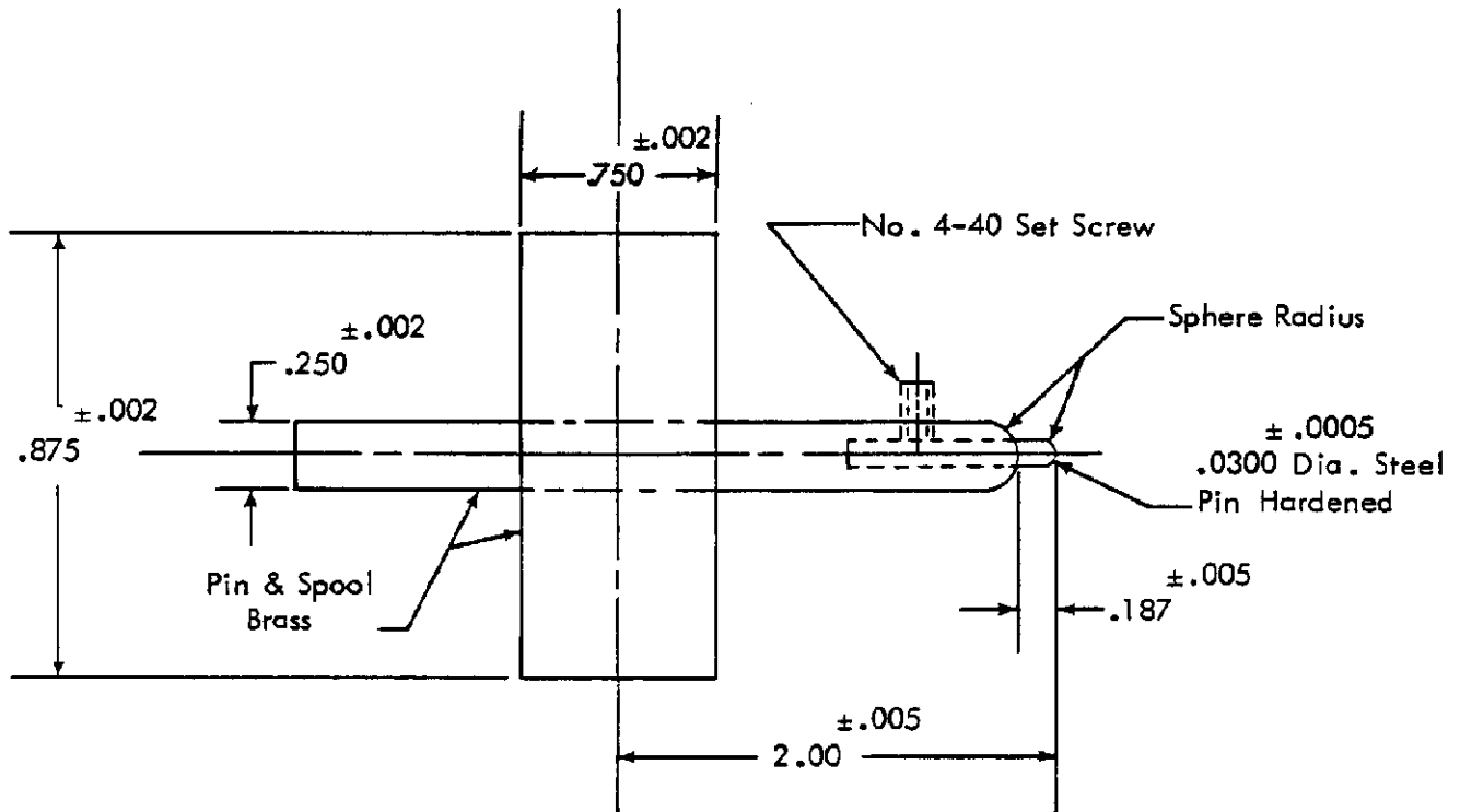
PROBE DAMAGE FIXTURE
