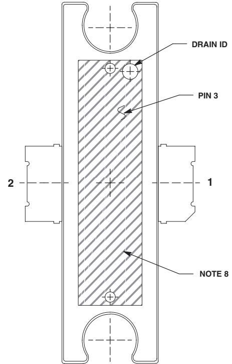
VIEW Y-Y
